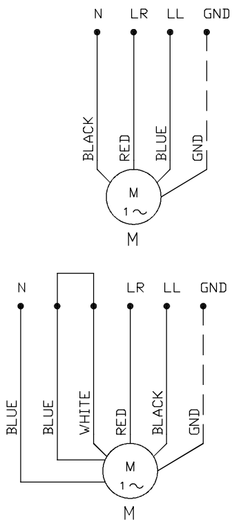
MOT310 TYPE MOTOR 1004.2456
