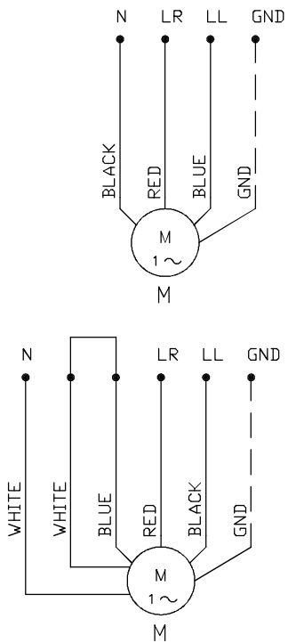
MOT310 TYPE MOTOR 1004.2456
